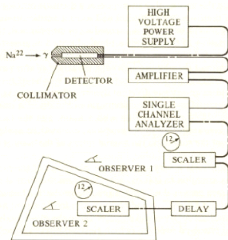
Figure 1. Hall's experiment
