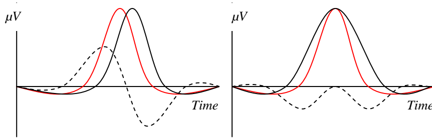
Figure 12. Example of difference waves (dashed) when two signals differ only in latency (left) or surface (right).
