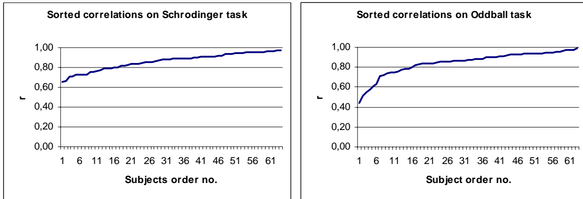
Figure 6. Correlation of subject's AEP trace with average AEP over all subjects. Note that the subjects are sorted by ascending correlation index r .
