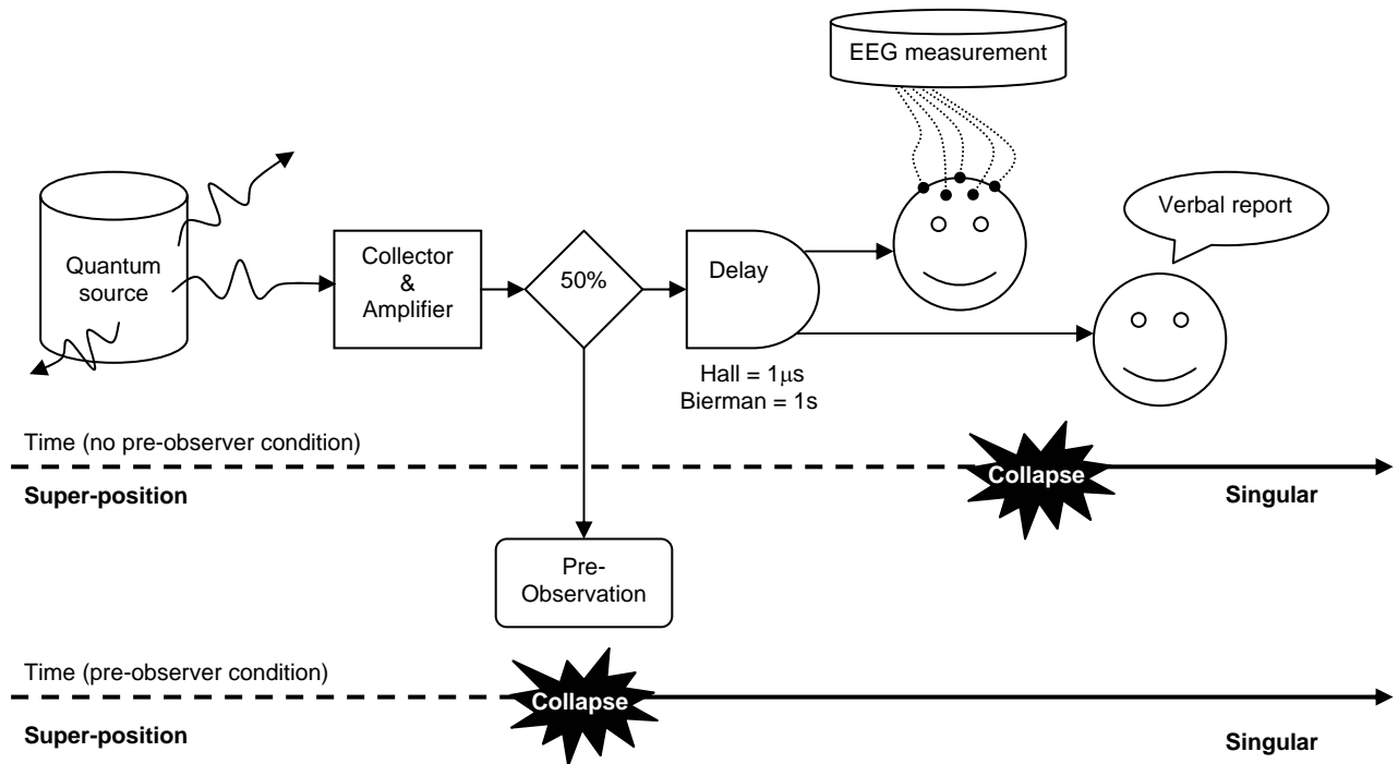
Figure 2. Design and time-line of the Hall experiment in which conscious report always occurs at the already singular state and the conscious measurement by EEG in super-position-time.
