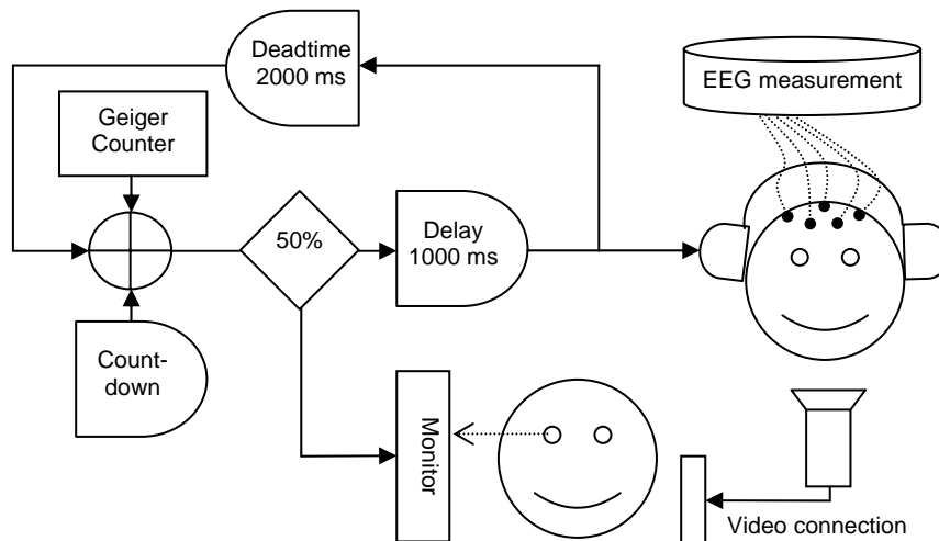
Figure 4. Experimental design. Note that the separated locations of the subjects are not shown. The crosshair depicts the alternating choice of quantum/classical event (absent in Bierman, 2003).
